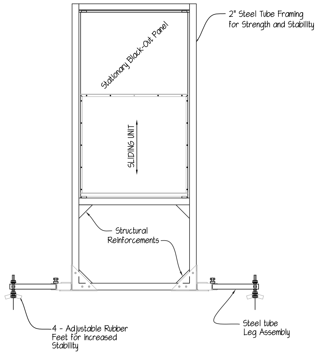
ELEVATION OF WINDOW WALL
