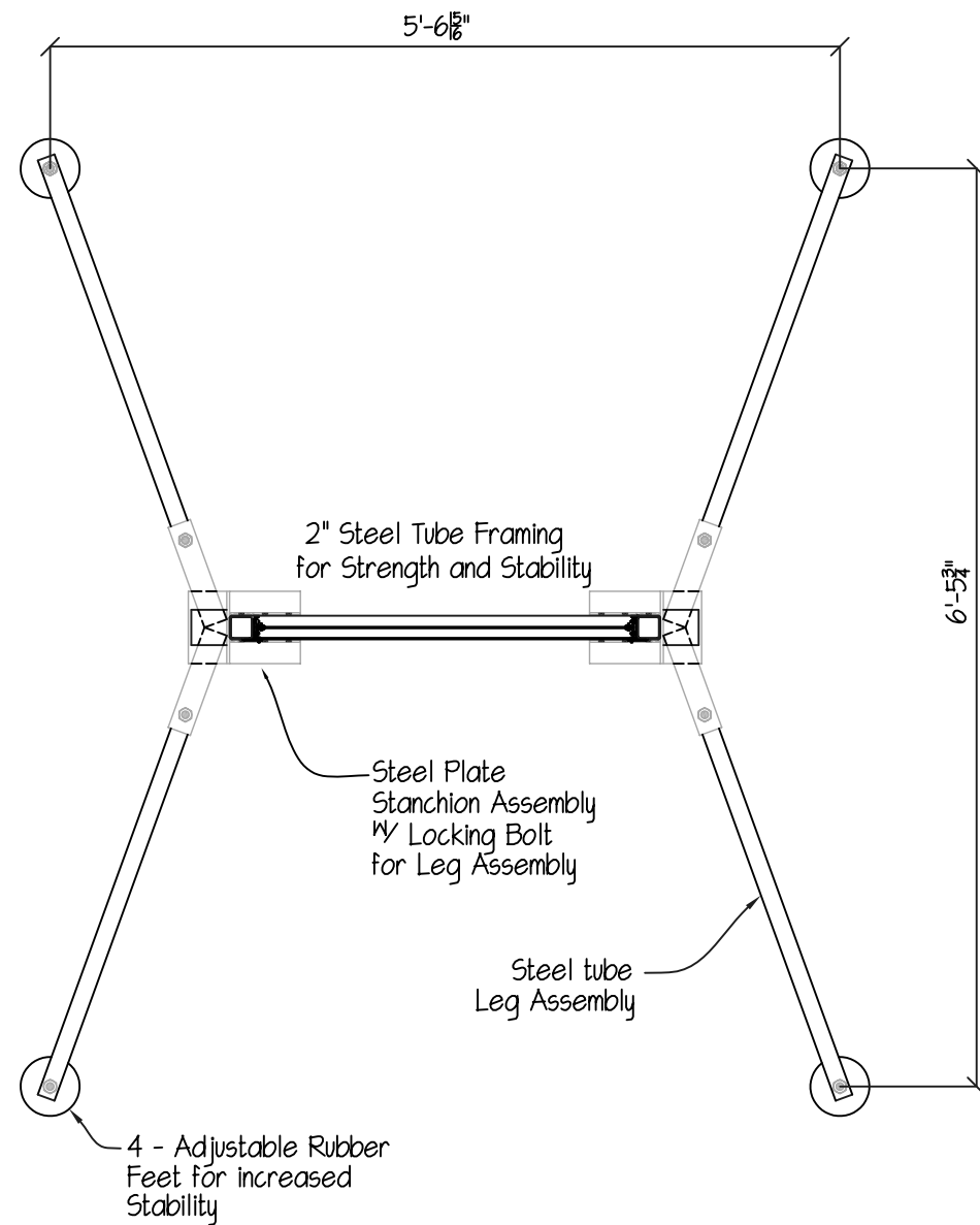
PLAN VIEW OF WINDOW WALL
