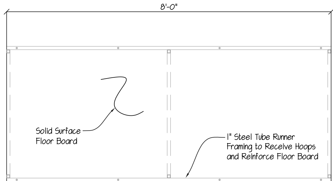
FRAMING PLAN
